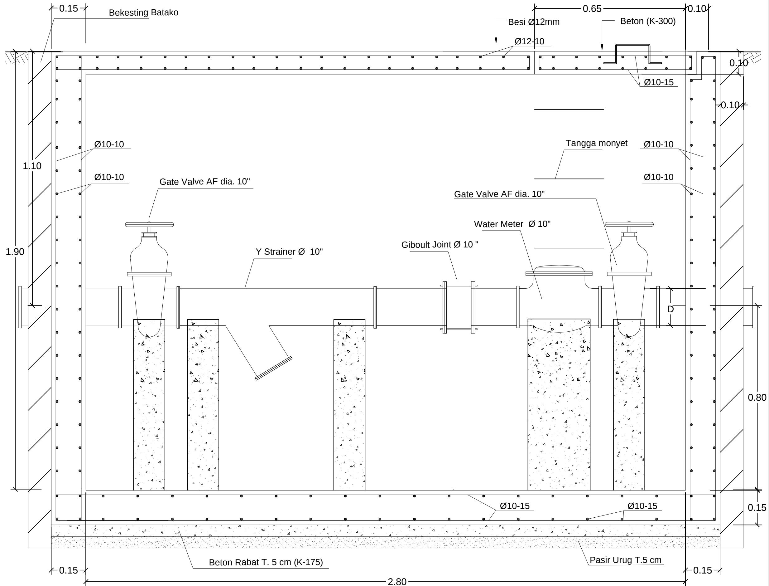
DETAIL POT. A SKALA 1 : 15
